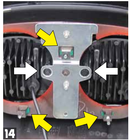
14 Now insert the Cyron headlight housing into the stock fairing aligning the two locating studs (white arrows) and three ball bolts (yellow arrows) with their holes in the fairing. Make sure both tabs on each of the three ball bolt clips lock into their supports.
