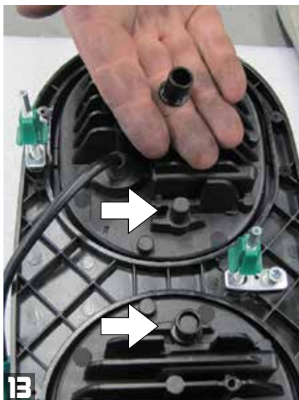
13 Then press the two black plastic Cyron-supplied collars onto the thick locating studs (arrows) on the new Cyron headlights.
